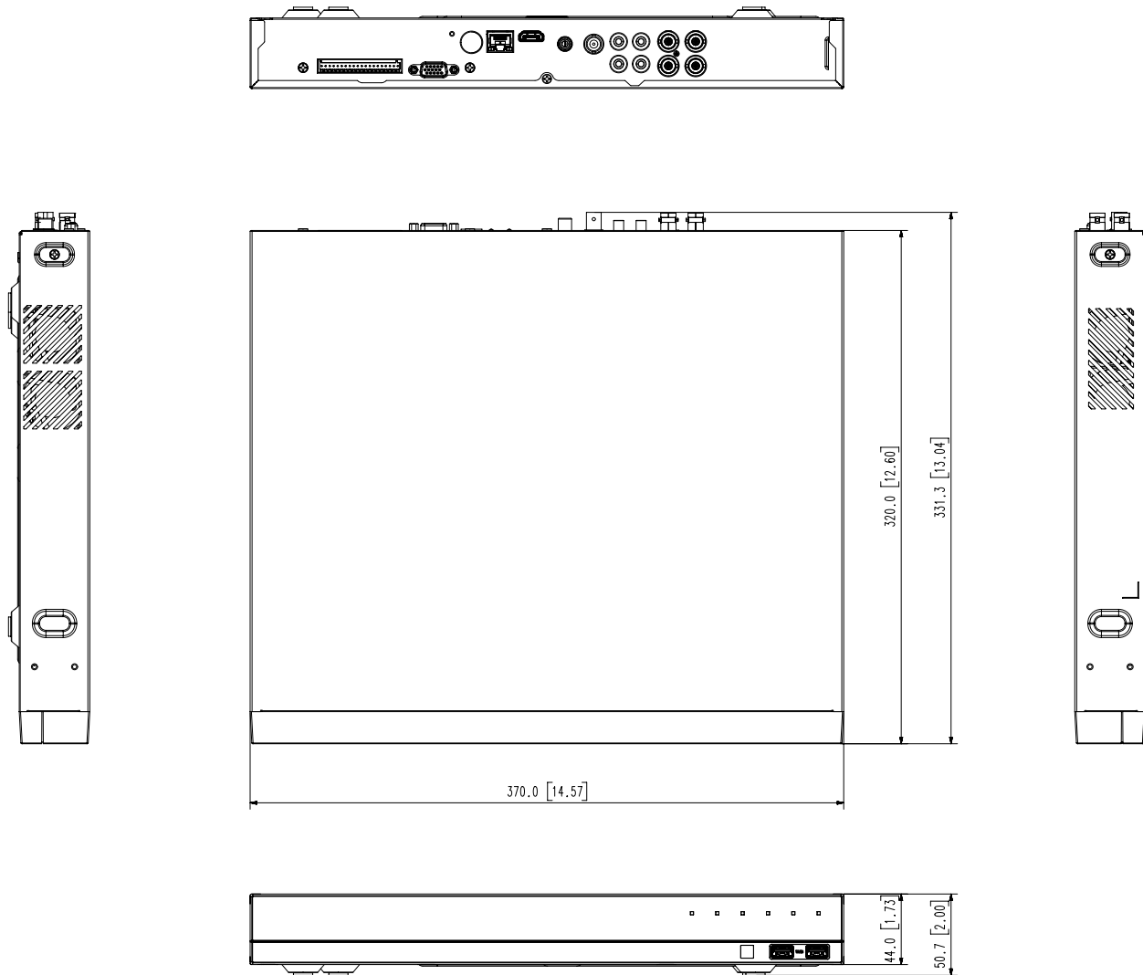
Appearance drawing HRX-421 Unit : mm[inches]
